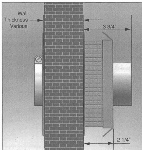
Fig. 7B: 3 Inch Vent Termination Dimensions
