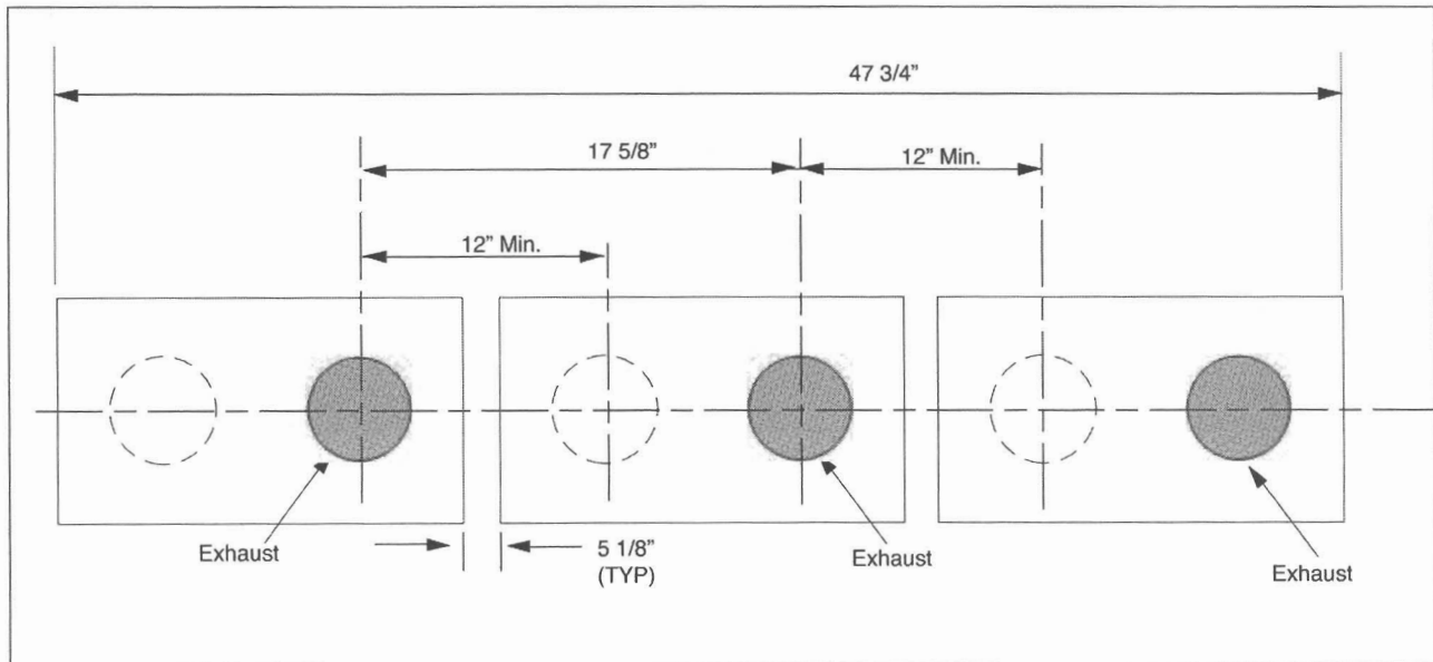
Fig. 6A: Multiple Horizontal Vent Installation 3 Inch Venting System
